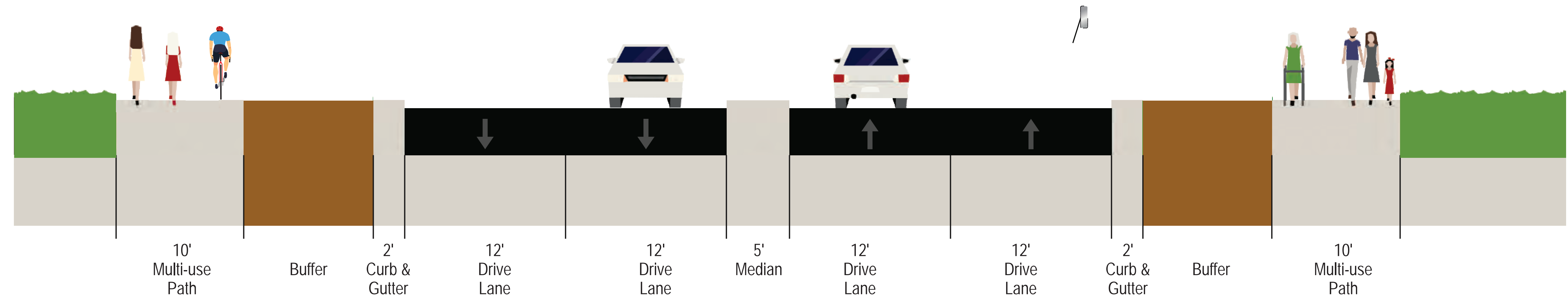
Orchard Street Cross Section | Approx 100' Right-of-Way
