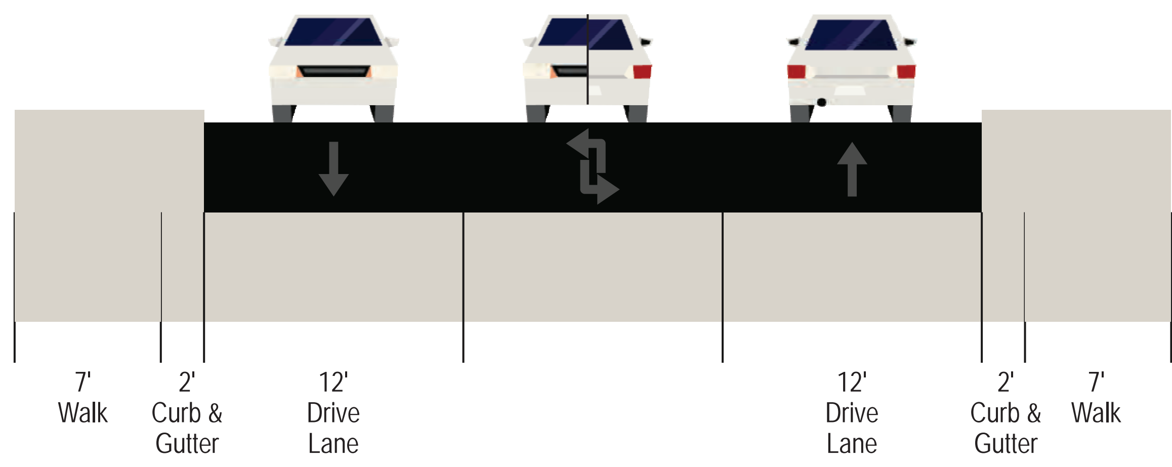
Alternative 2 Dorman Street Connector | Approx. 58'
